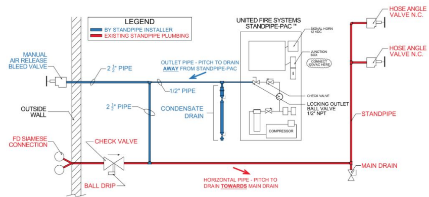
STANDPIPE-PAC™ FIELD CONNECTIONS
