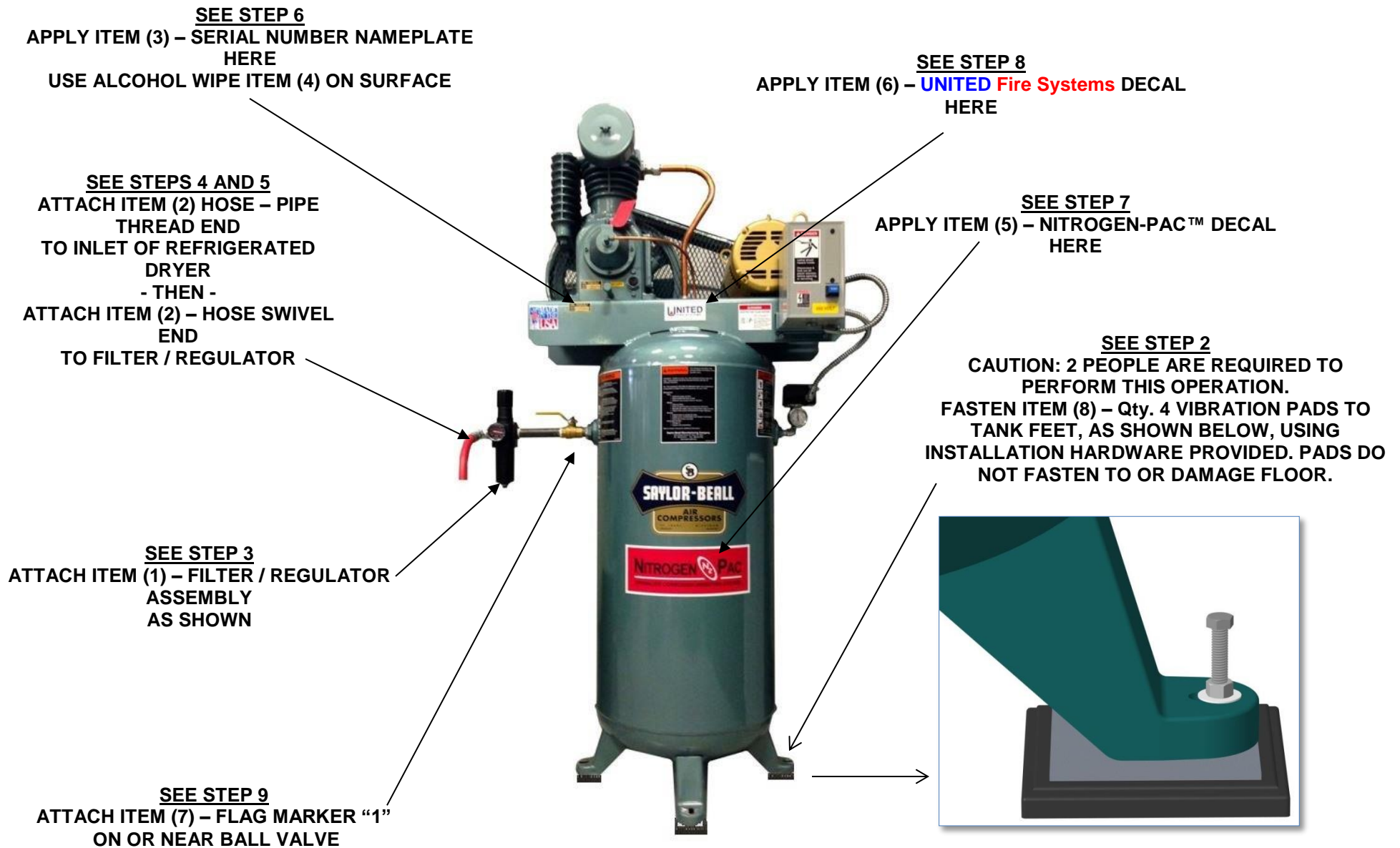
FIGURE B – LOCATIONS OF INSTALLATION KIT ITEMS
