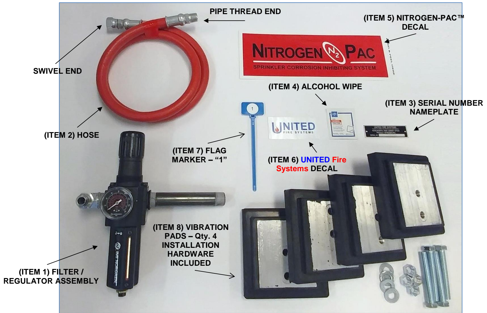
FIGURE A – CONTENTS OF INSTALLATION KIT
