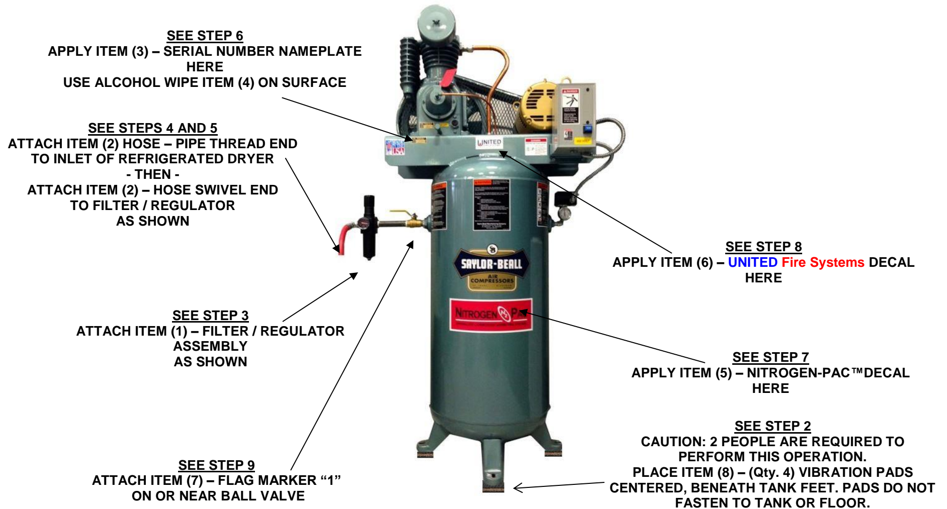
FIGURE B – LOCATIONS OF INSTALLATION KIT ITEMS
