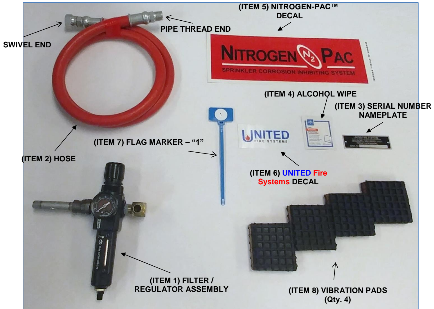
FIGURE A – CONTENTS OF INSTALLATION KIT
