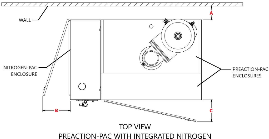
Figure 3 – Required Clearances
