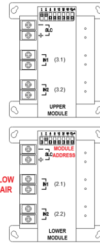
Figure 3 Low Air Switch Wiring Potter ARC-100 Control Panel
