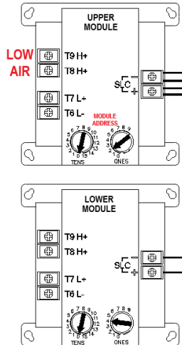
Figure 1 Low Air Switch Wiring Notifier NFS2-640 & INSPIRE Control Panels
